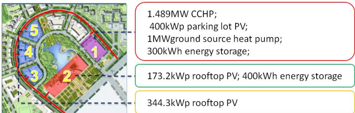
Figure 9: Diagram of the Microgrid Serving the Eco-City Animation Park
