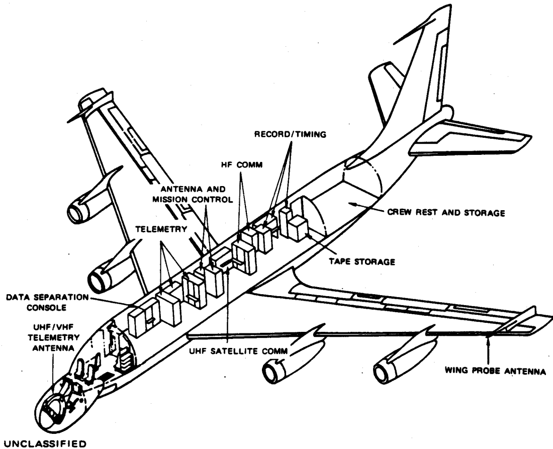
FIGURE 18 (U) ARIA INTERIOR MODIFICATIONS
