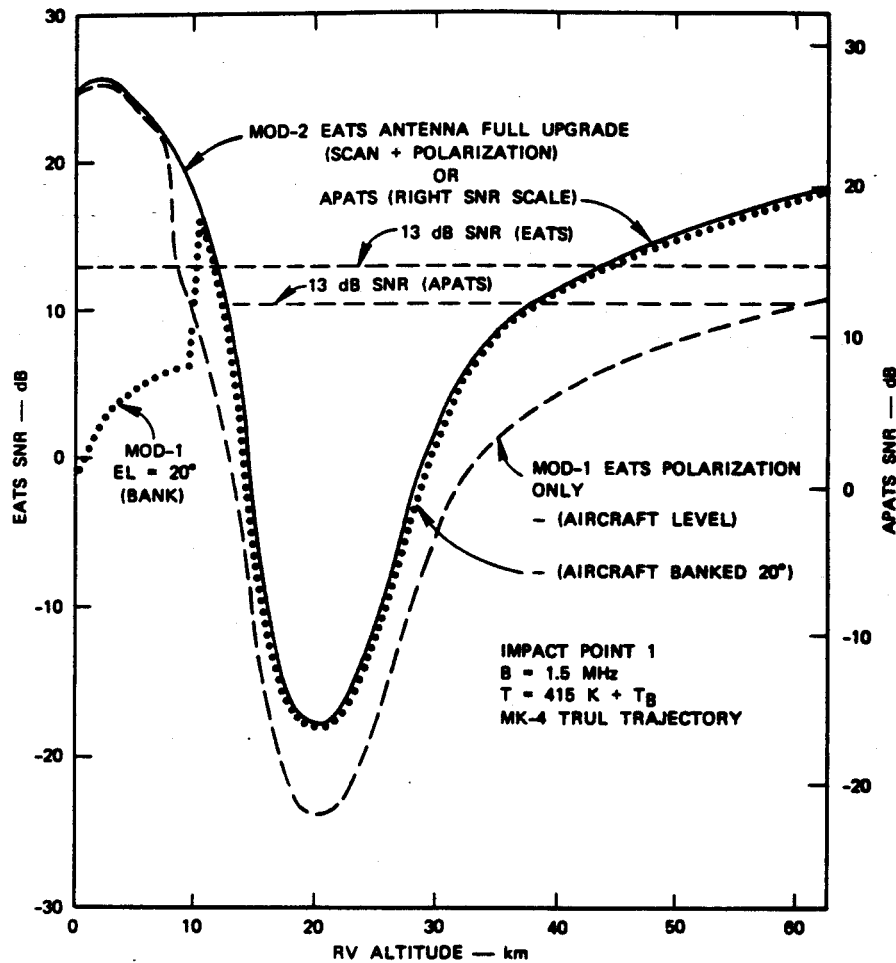
FIGURE 47 (U) EATS AND APATS ANTENNAS WITH MK-4 RV TELEMETRY
