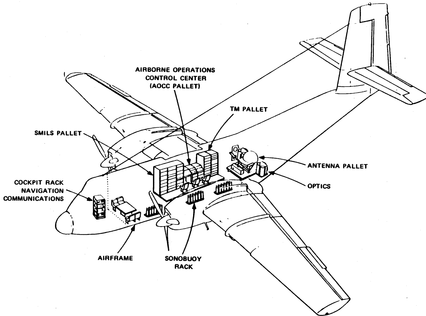
FIGURE 36 (U) C-7A TASA DESIGN CONFIGURATION
