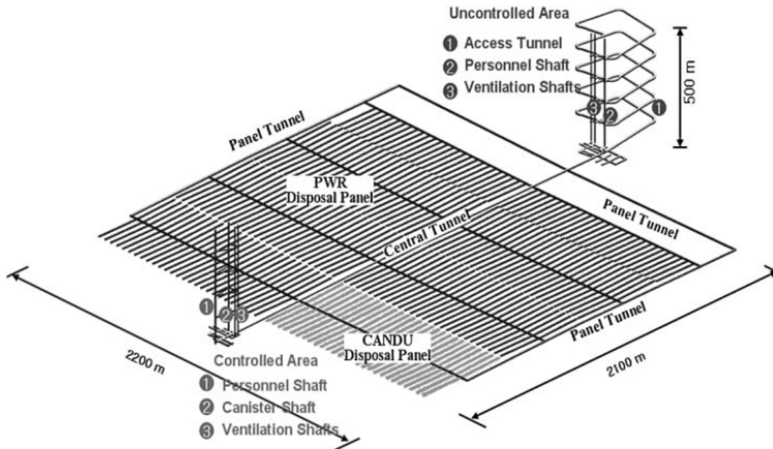
Figure 7: Layout of the Korean Reference Disposal System
