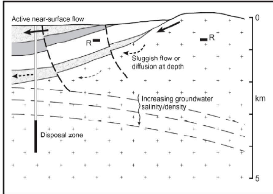
Figure 1: Conceptual Model for Deep Borehole Disposal
