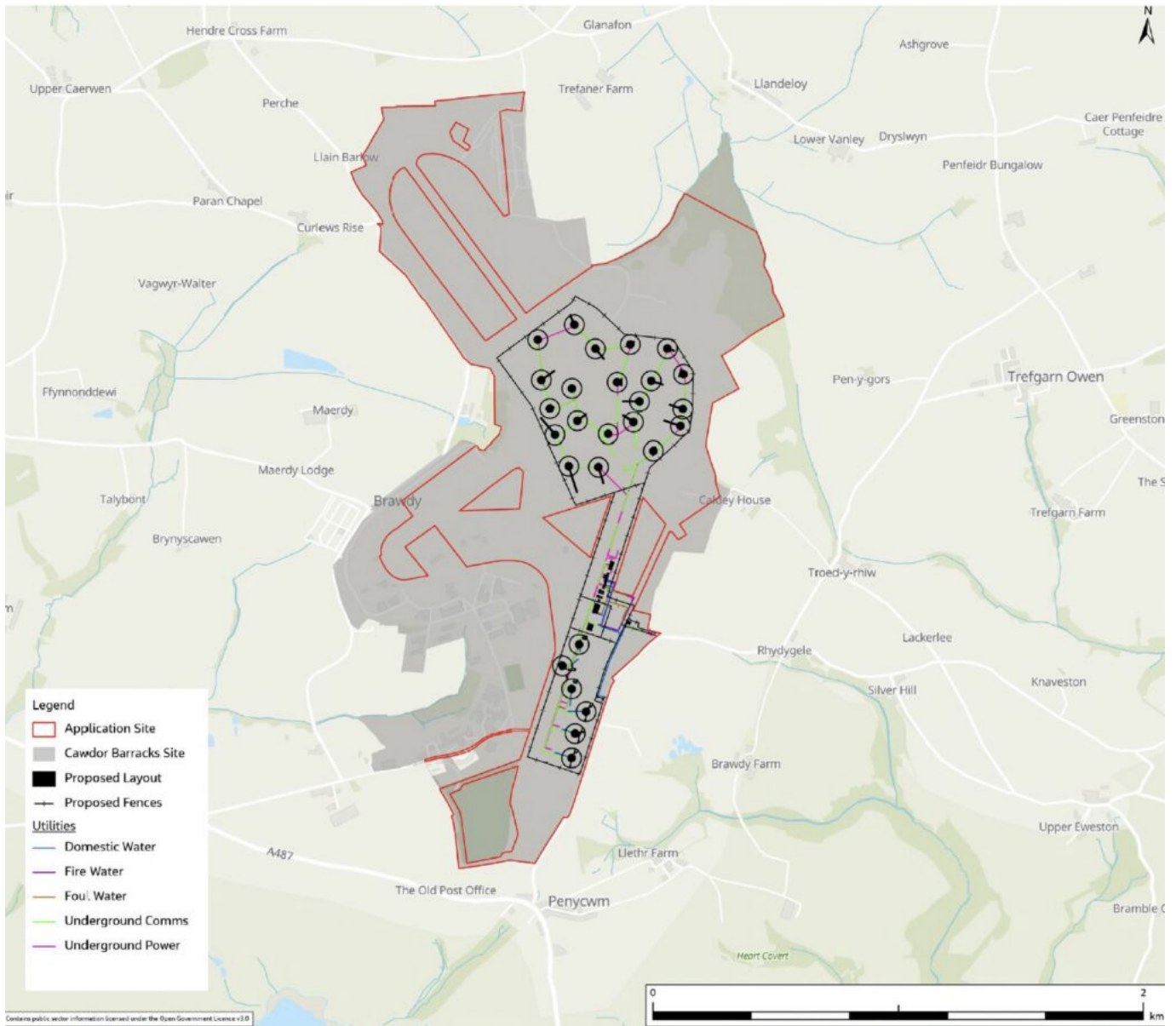
Planned layout of DARC Site 2 antenna arrays: receive array (north) and transmit array (south)
