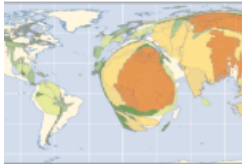
Major shifts from 1976 to 2010 (February) based on ESM GISSER2
