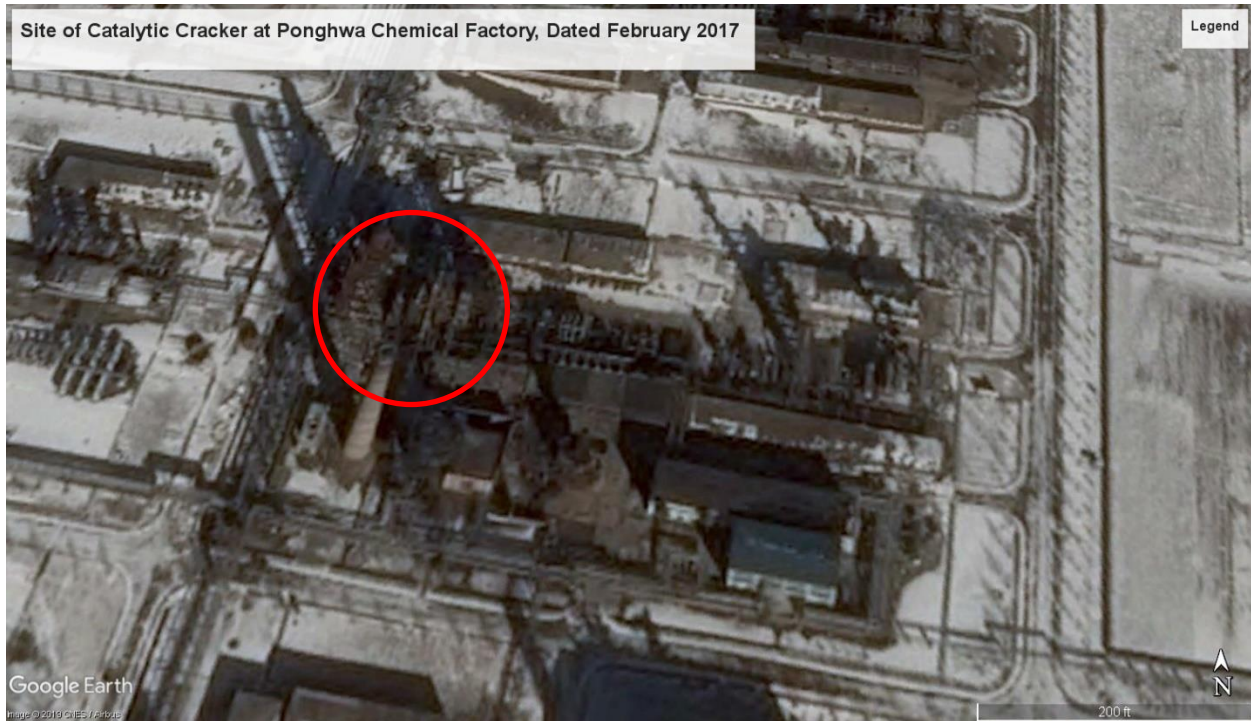
Figure 13: Probable Catalytic Cracking Unit at Ponghwa Chemical Factory as of February 16, 2017 21
