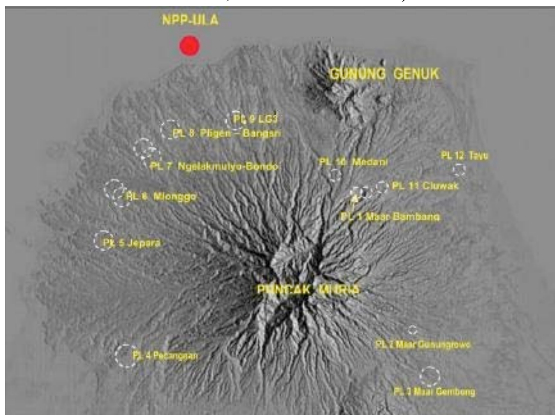
Figure 4. Volcanic maars on the Muria Peninsula (from Sutikno Bronto dan Sri Mulyaningsih, "Gunung api maar di Semenanjung Muria", Jurnal Geologi Indonesia , Vol. 2 No. 1 Maret 2007.)
